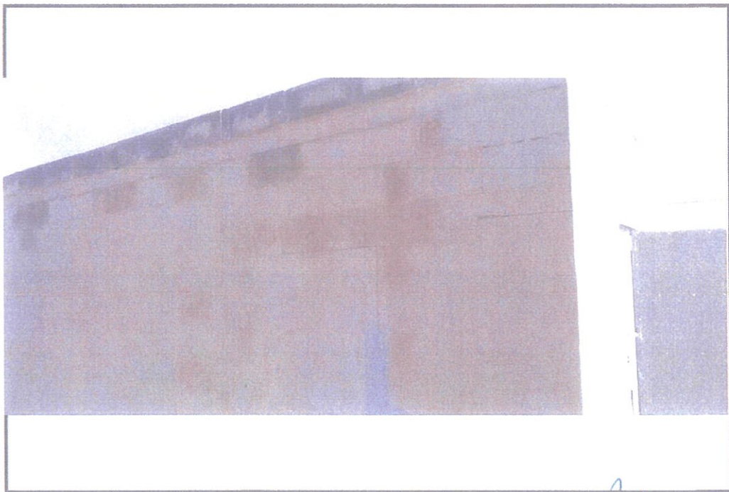
PHOTO NO.6-- Multiple external wall cracks on stairwell at roof level
