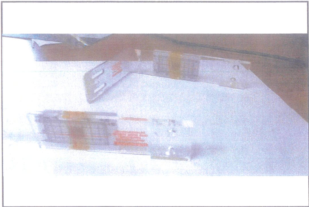
PHOTO NO. 16 - Plastice "Tell Tales" to monitor wall deformation across wall cracks
