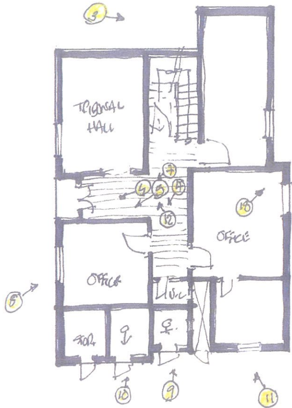
GROUND FLOOR PLAN/SKETCH @ 1:100 SCALE
