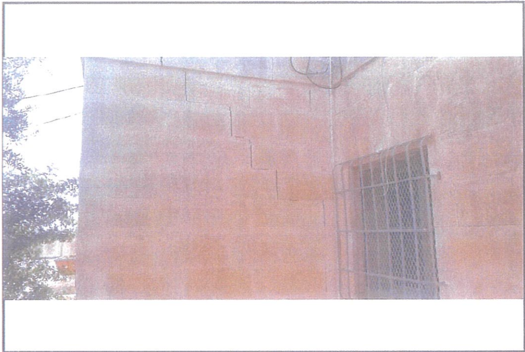
PHOTO No.3 -- Visible Rotaional Wall Crack ( Konsentura ) as seen on facade
